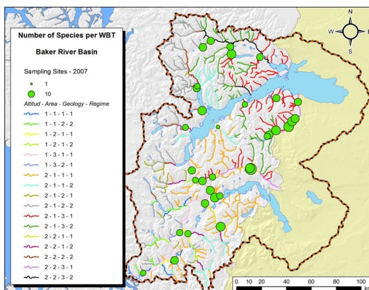
Figure 5. Species richness at the different sampling sites. Background shows the water body typology determined under Work Package 7.
