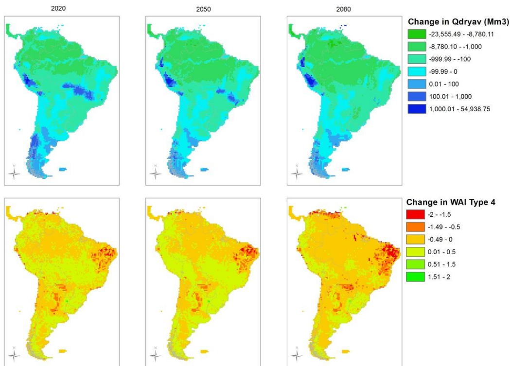
Figure 100. Changes in the low flow index (above) and WAI 4 (below) for 2020, 2050 and 2080.
