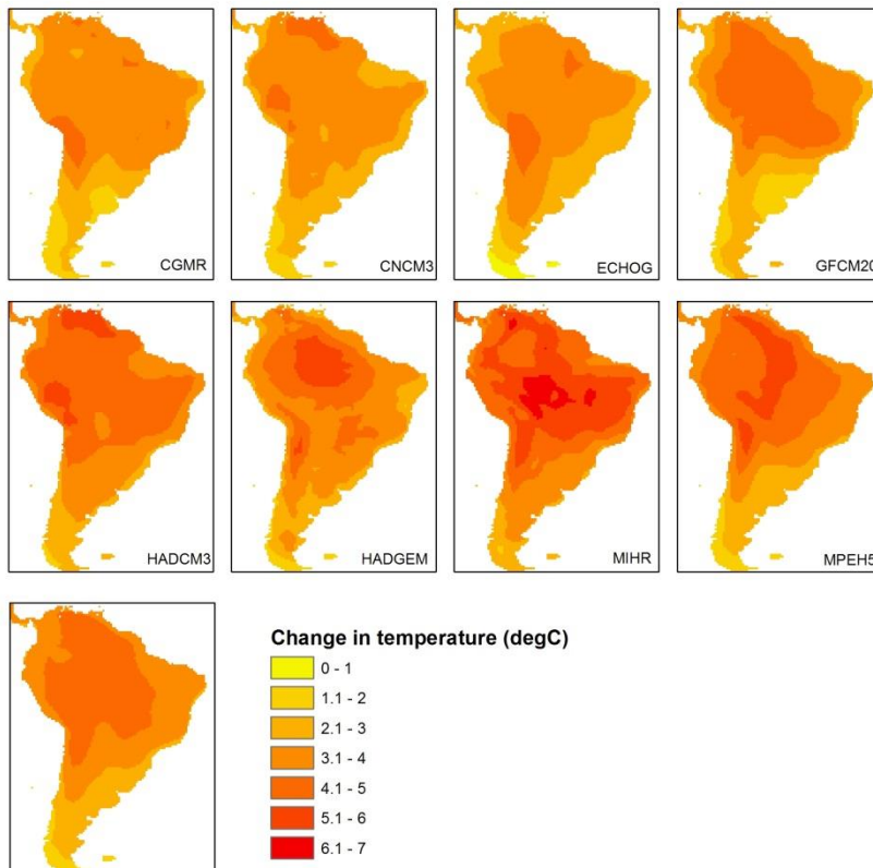
Figure 98. Absolute change in annual air temperature for eight GCMs (A1B scenario) and mean change of the eight models (bottom left)
