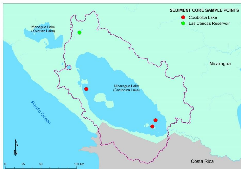
Figure 12. Sites in the Cocibolca Lake Basin where the sediment cores have been taken
