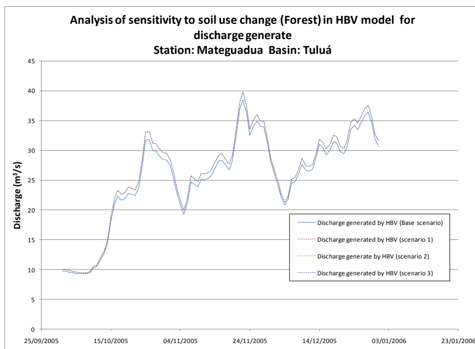
Figure 80. Predicted effects of de/afforestation in the Tuluá river basin
